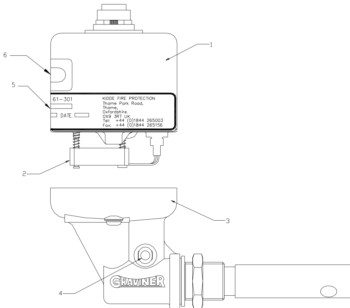
Figure 52 Detector Head E3561-301
